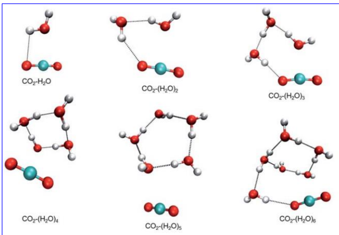
FIG. 7. QM-optimized structures of CO 2 -water clusters with various numbers of water ligands from n = 1 to n = 6 .
