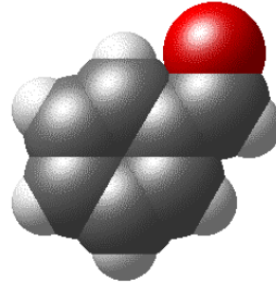
Benzaldéhyde
